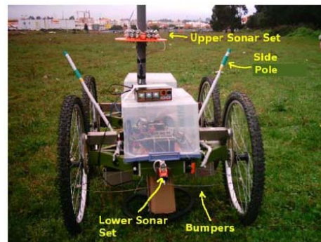
Figure 3: Four-Wheeled System[6]
